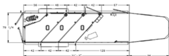
Floorplan: 3-horse with 67" dressing room
