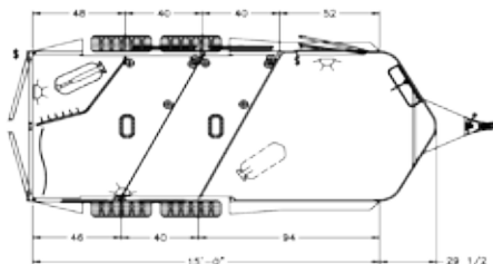
Floorplan: 2-horse with 52" dressing room, 7' width and 40" stalls.
