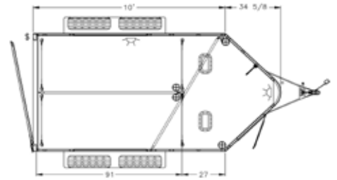
Floorplan: 2-horse Photos: 2-horse
