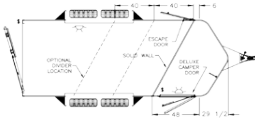
Floorplan: 7' wide slant wall combo conversion Photo: 12' length
